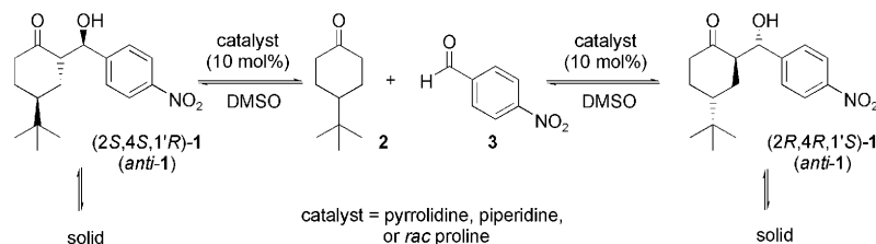
Scheme 1. Catalytic enantioenrichment of aldol product anti -1 in presence of achiral or racemic secondary amines.
