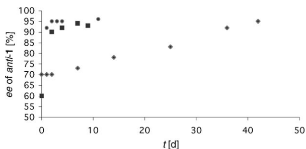
Figure 1. Enantiomeric excess of anti -1 versus reaction time in the enantioenrichment shown in Scheme 1. Catalyst/starting ee of anti -1 (for details see text): pyrrolidine 70% (●); pyrrolidine 60% (■); rac -proline 70% (◆).
