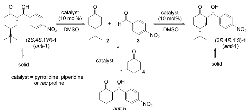
Scheme 2. Enantioenrichment of aldol product anti -1 in presence cyclohexanone ( 4 ) as co-reactant.
